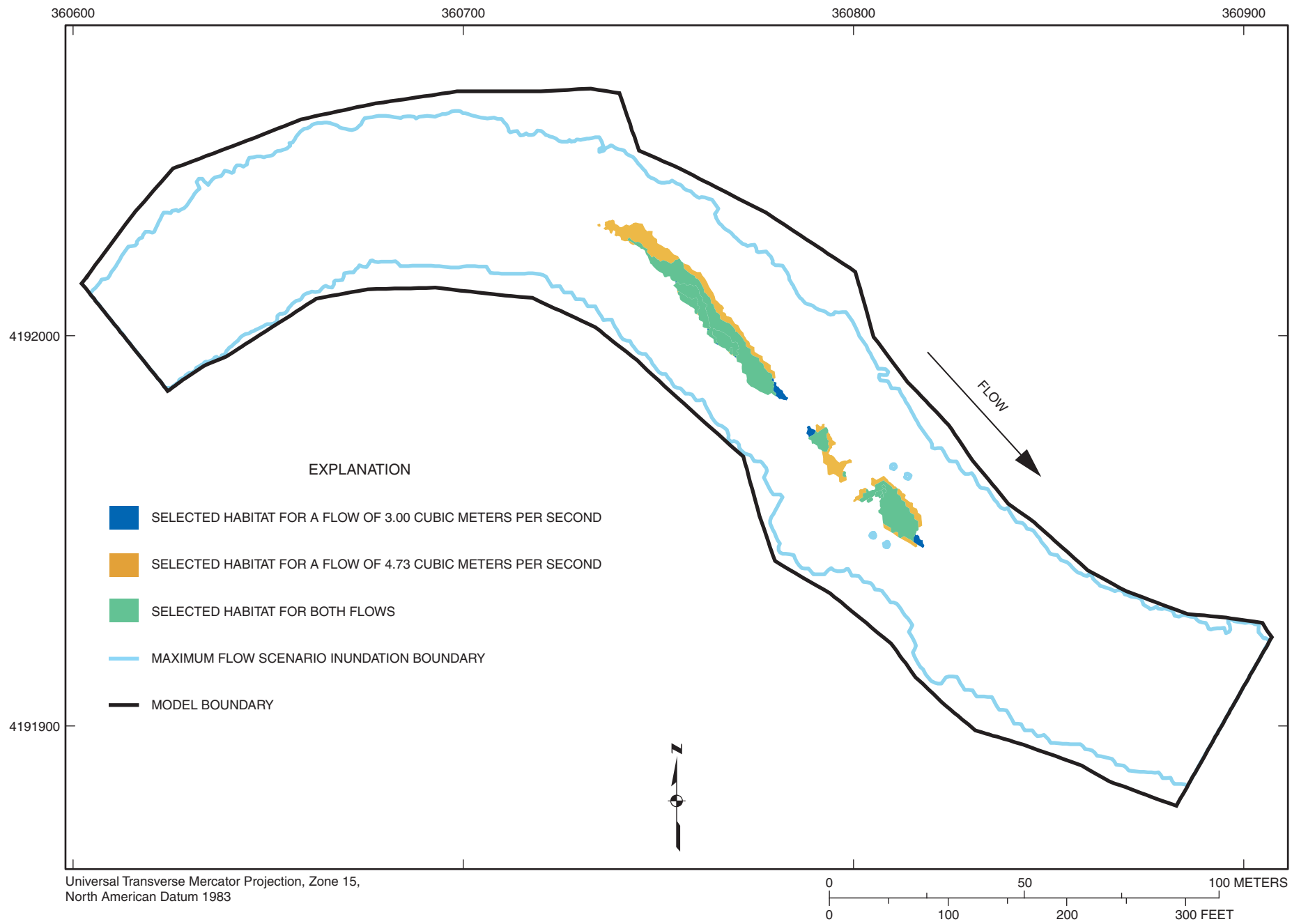
Figure 1-9. Selected habitat area distribution for habitat categories 4, 5 combined (slenderhead darter) at flows of 3.00 and 4.73 cubic meters per second at Marmaton River site M1.
